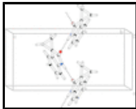
Fig. 2. Part of the crystal structure with hydrogen bonds shown as dashed lines.
